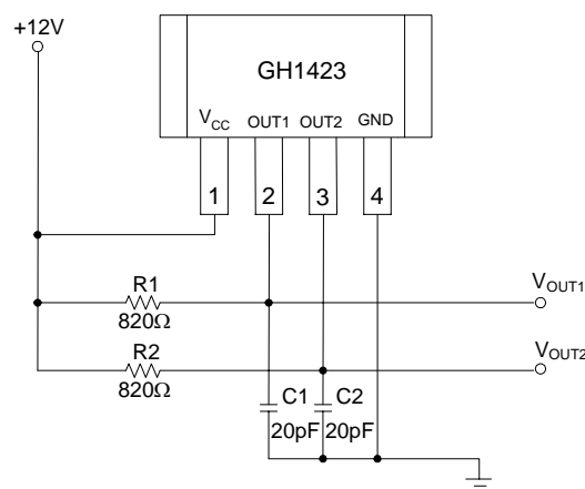
Fig 3. Test Circuit
