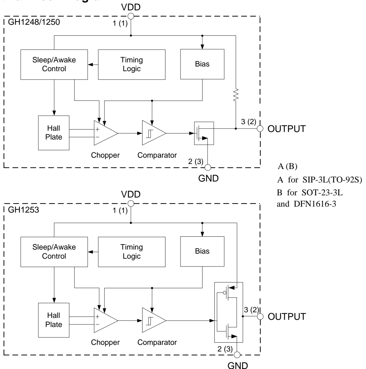
Figure 3. Functional Block Diagram of GH1248/1250/1253
